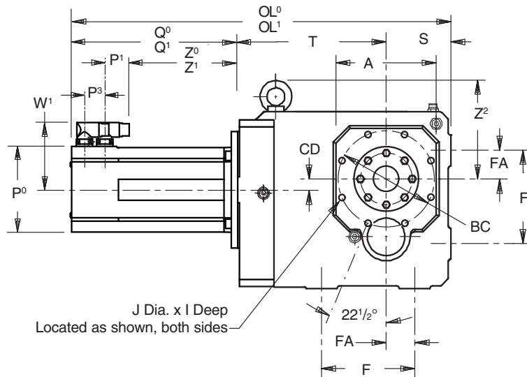
Drawing for Units K513WG — K814WG
