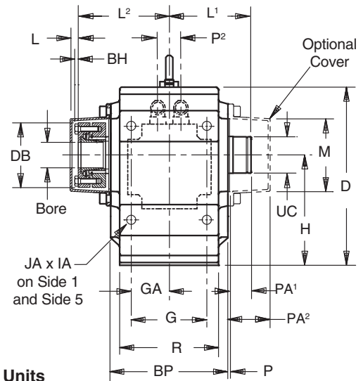
Drawing for Units K513WG — K814WG
